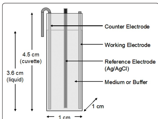
Figure 1 Schematic of the electrochemical cell used in this study. The reference electrode is Ag/AgCl wire inserted in a thin glass tube to prevent contact with the working or counter electrode. Biofilms grown on flat steel or carbon electrodes can be clipped onto the side; the liquid level is about 1 cm below the top of the cuvette when full (3 mL).
