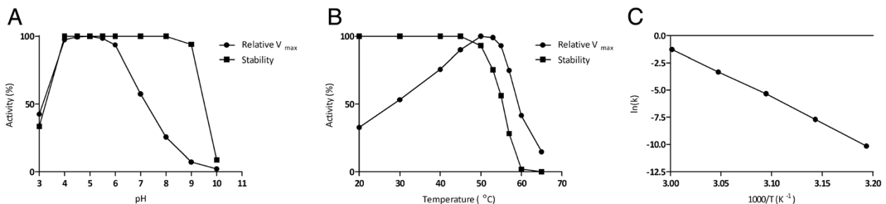
Figure 2 Temperature and pH parameters of BXA43. (A) Stability (■) and activity (relative V_{max} ) (●) pH profiles of BXA43 using pNPX as substrate. (B) Stability (■) and activity (relative V_{max} ) (●) of BXA43 as a function of temperature using pNPX as substrate. (C) Arrhenius plot of the effect of temperature on the t_{1/2} for thermal inactivation of BXA43 in the temperature range 40–60°C (see Methods for details).
