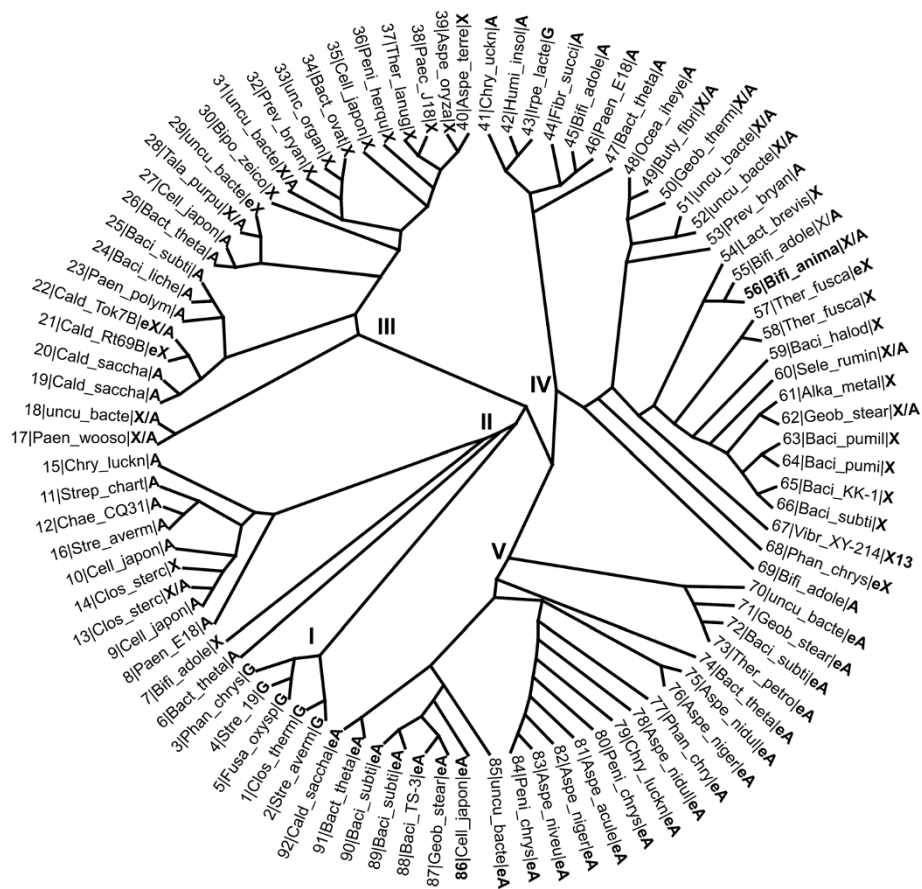
Figure 1 Phylogenetic tree of GH43 enzymes annotated as characterised in the CAZY database (prepared by Dendroscope). Five distinct groups (I-V) are observed which represent different specificity clusters. BXA43 (in bold ) is found in group IV. Enzyme activities have been abbreviated as X: \beta -D-xylosidase (EC 3.2.1.37). X13: \beta -1,3-xylosidase (EC 3.2.1.-). A: \alpha -L-arabinofuranosidase (EC 3.2.1.55). eA: endo-arabinanase (EC 3.2.1.99), eX: endo-xylanase (EC 3.2.1.8). G: galactan 1,3- \beta -galactosidase (EC 3.2.1.145). The entries are numbered and further details like the full organism names and UniProt identifiers can be found in Additional file 1: Table S1.
